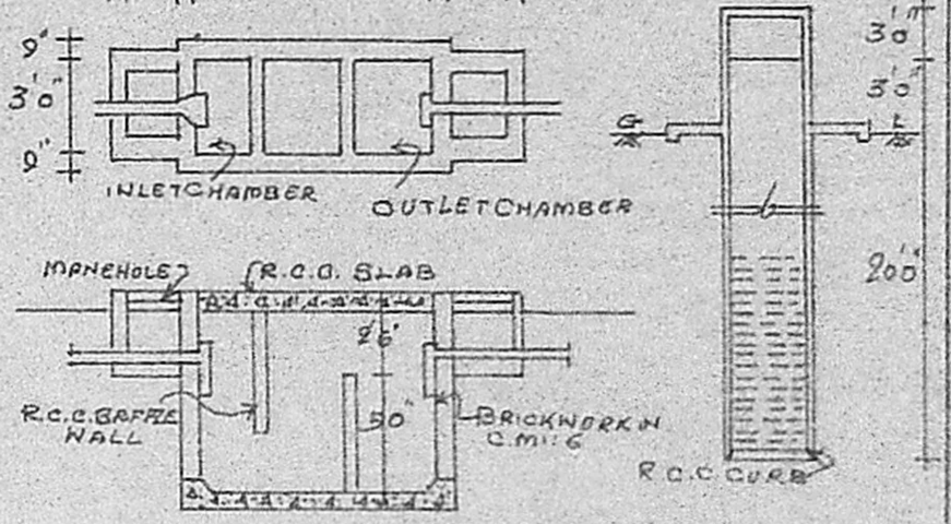
DETAILS OF SEPTICTANK & DIA WELL
