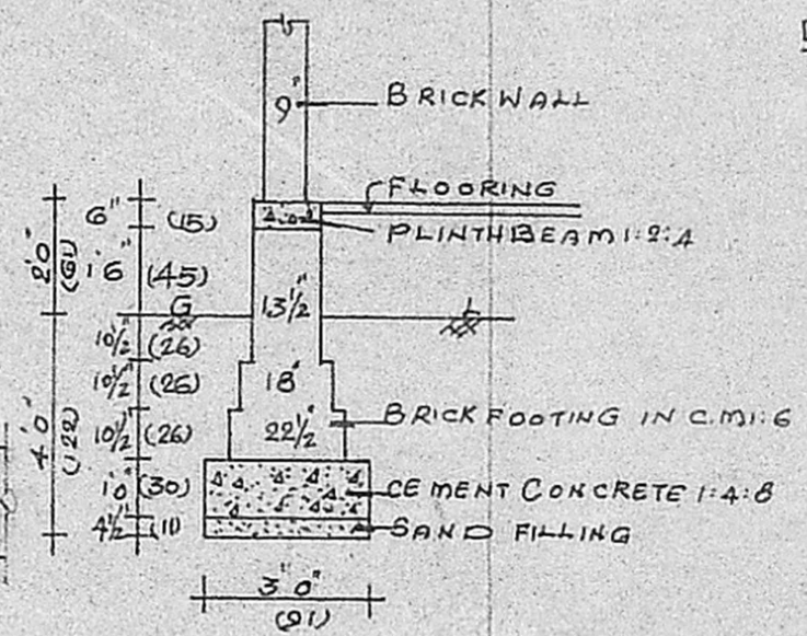
FOUNDATION DETAILS
